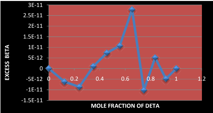
Fig 9 Graph between variation of excess adiabatic compressibility and mole fraction of DETA in 1-Chloronapthalene at constant temperature and fixed ultrasonic frequency
