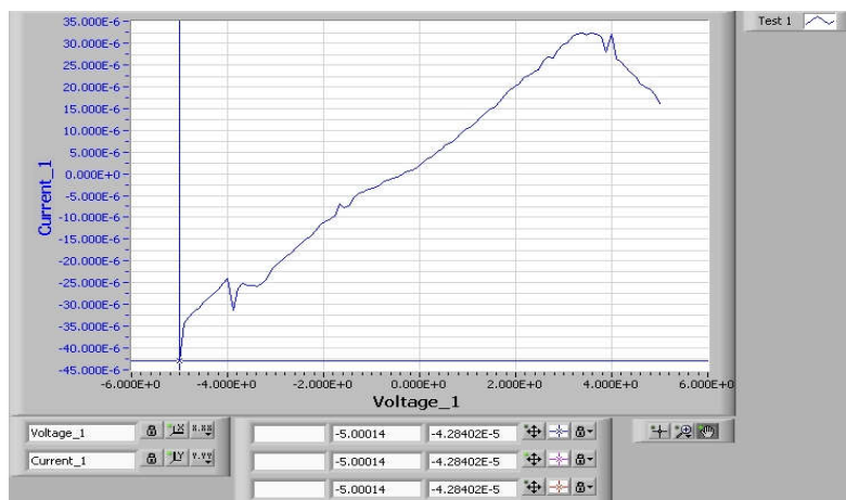
Figure 3: Electrical conductivity of Graphene/Polyaniline sample J1 using two probe system at first positions.
