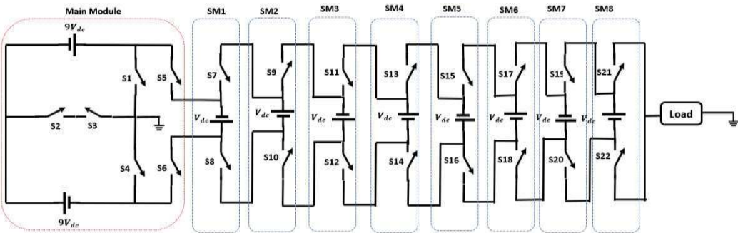
Fig.9 53 level inverter
