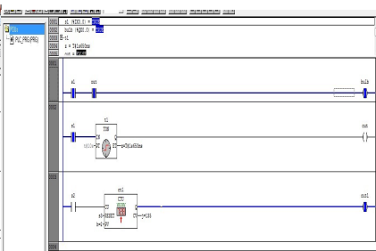
Figure 2 Ladder diagram-level 2
