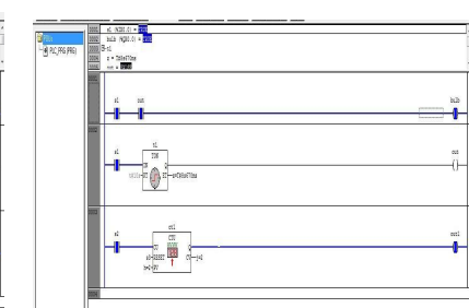
Figure 3 Ladder diagram-level 3
