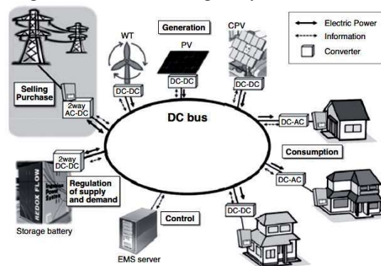
Figure 1: Schematic diagram of a DC microgrid system
