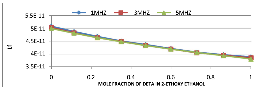
Fig 2 Graph between variation of intermolecular free length & mole fraction of DETA in 2-Ethoxyethanol at constant temperature 296K and frequencies 1MHz, 3MHz & 5MHz
