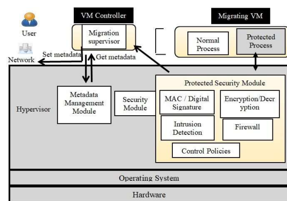
Figure 1: Protected Secure Live Migration
