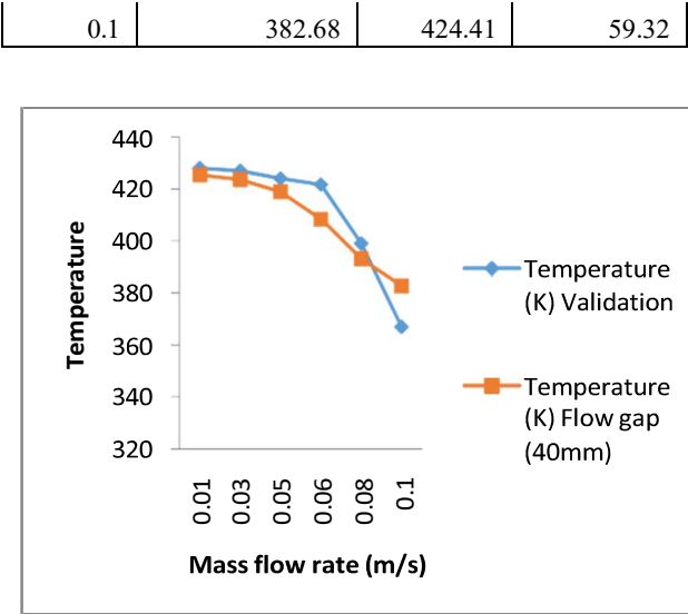
Figure - Temperature distribution of solar panel photovoltaic with water flow gap of 40mm.
