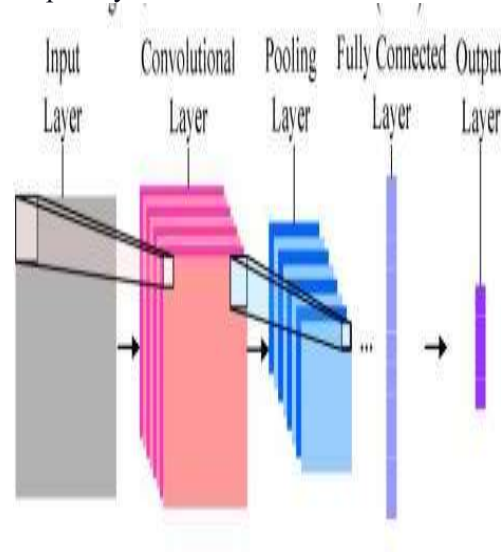
Fig 1 CNN Layers
